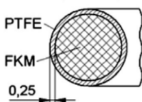
Detail X
